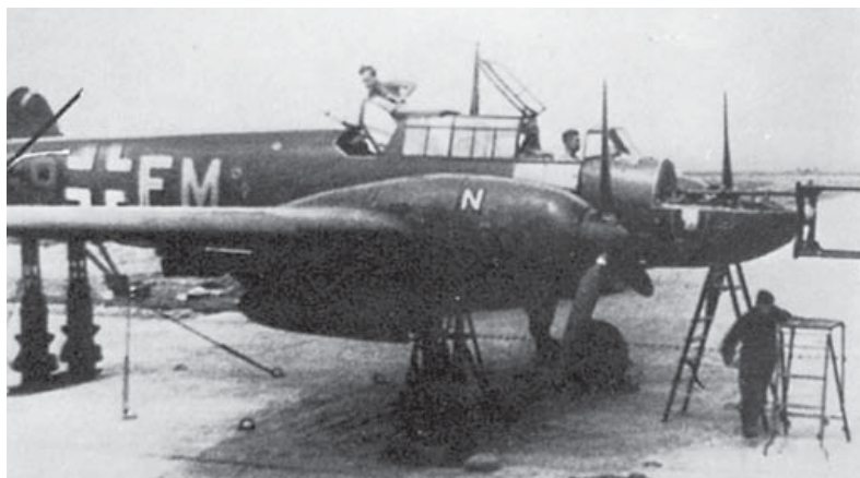
A Bf 110F-4 of 4./NJG 1 undergoes servicing on the ramp at St Trond airfield, in Belgium, during the summer of 1942. This aircraft has been fitted with FuG 202 Lichtenstein aerial intercept radar, the system's antenna array clearly visible forward of the nose. The "N" on the engine cowling denotes that the fighter is powered by a pair of DB 601Ns. (via Jerry Scuttis)
